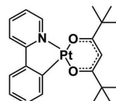
(ppy)Pt(dpm)
