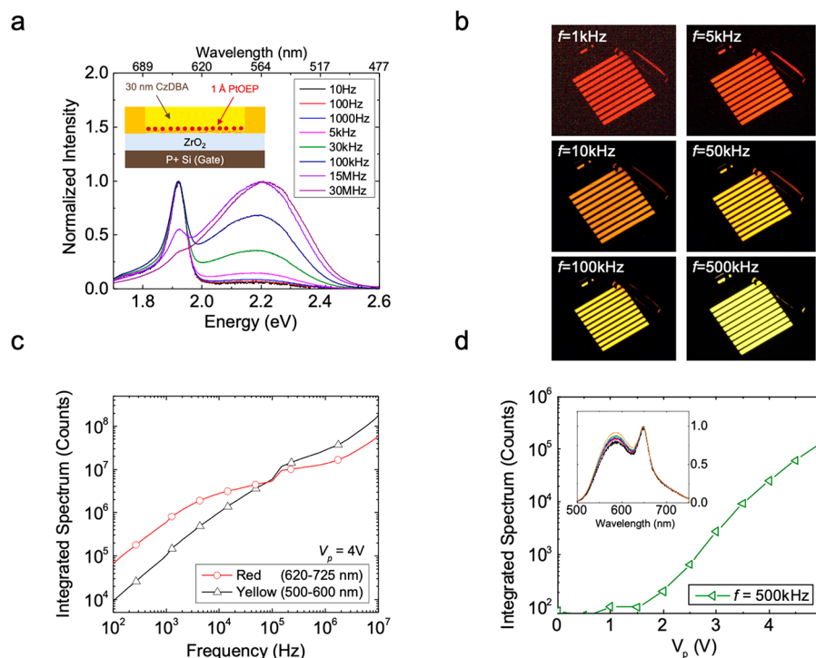
Figure 2. (a) Frequency dependent spectra of the color tunable device. Inset : schematic illustration of the device structure. (b) Photographic image of the device electroluminescence at varied frequencies. (c) Integrated spectrum of different color regions at varied AC frequencies. (d) Voltage dependent integrated spectrum. Inset : voltage dependent spectrum of the device.
